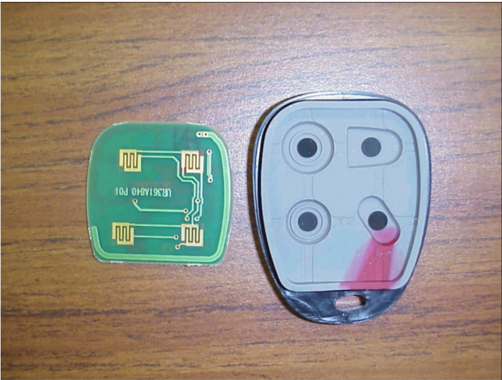
Delphi-Delco PCB - Key Side
