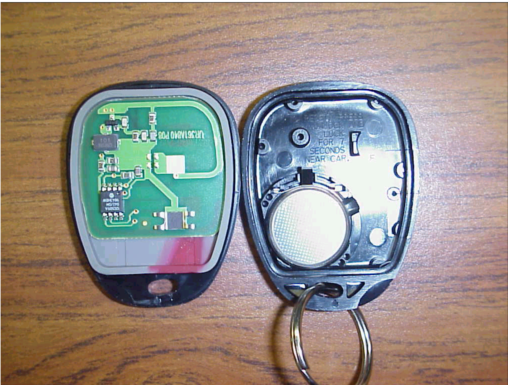
Delphi-Delco PCB with Battery
