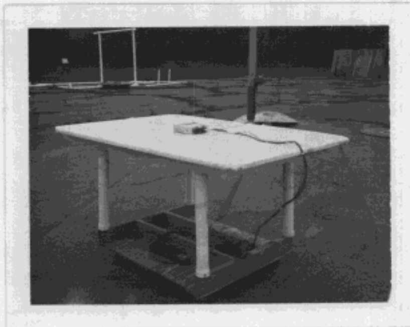
Figure 5.4. DUT on the open-site test table showing the worst case position and orientation with respect to the measuring antenna at "fundamental".
