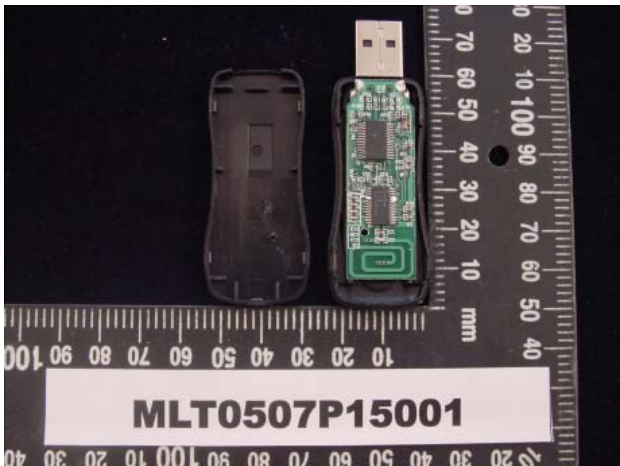
Inside View of Receiver
