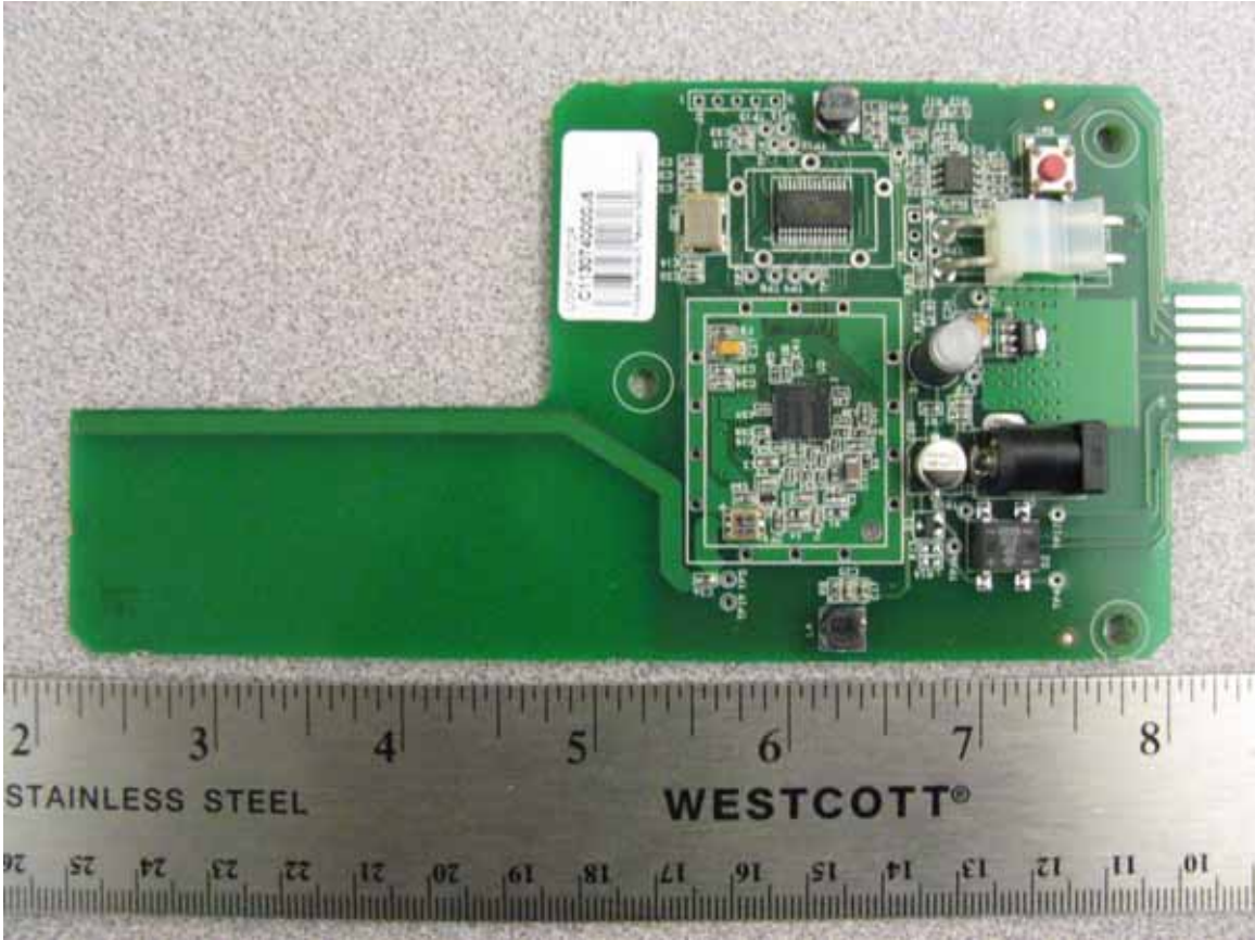
Monitor board component Side View
