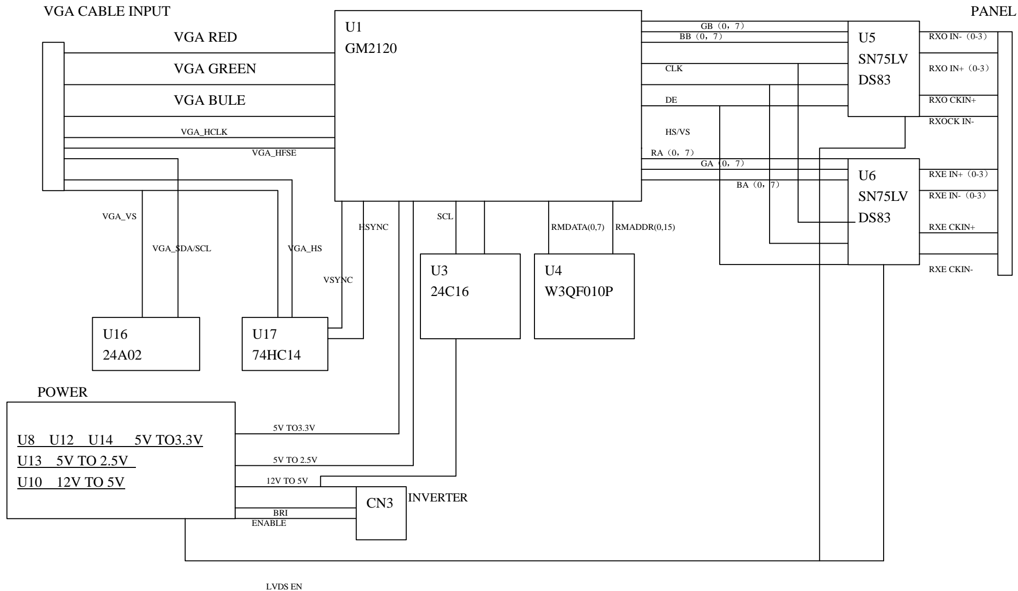
NV721C BLOCK DIAGRAM
