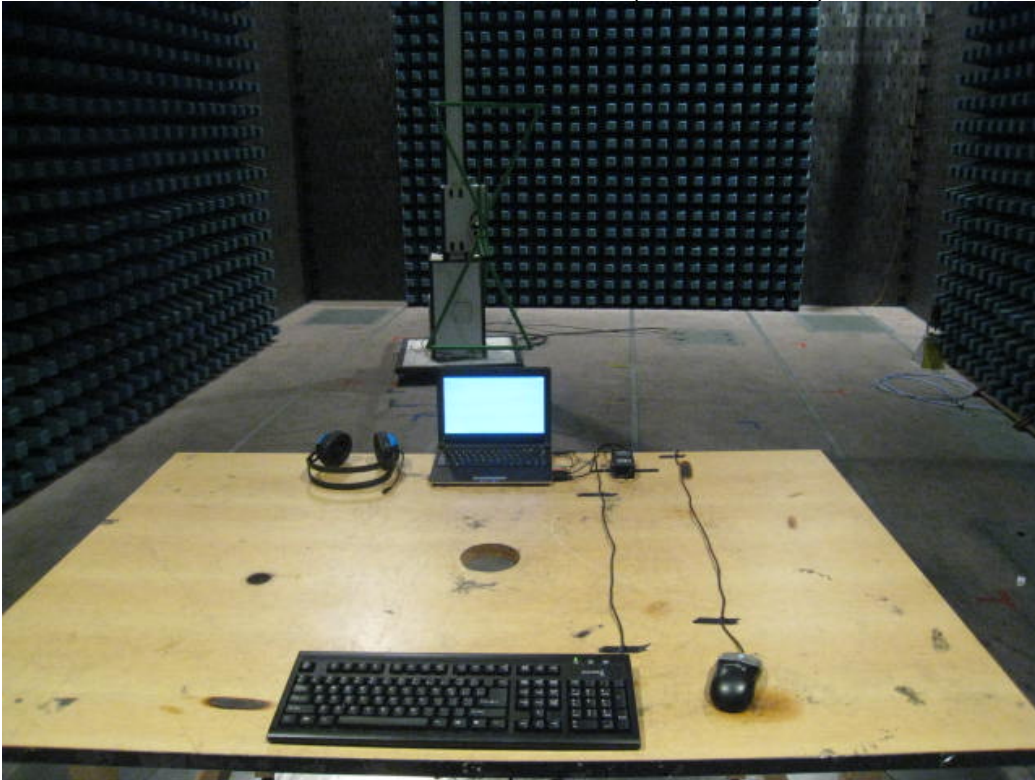
Photo 3 Front of Radiated Disturbance Test (Below 1GHz)
