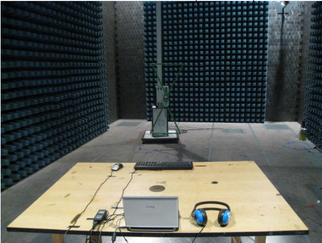
Photo 4 Rear of Radiated Disturbance Test (Below 1GHz)
