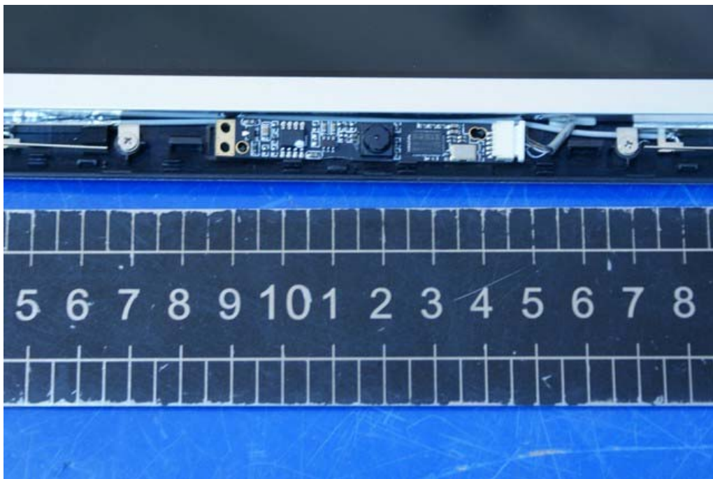
Photo 2 Inside of EUT (with Antennae)
