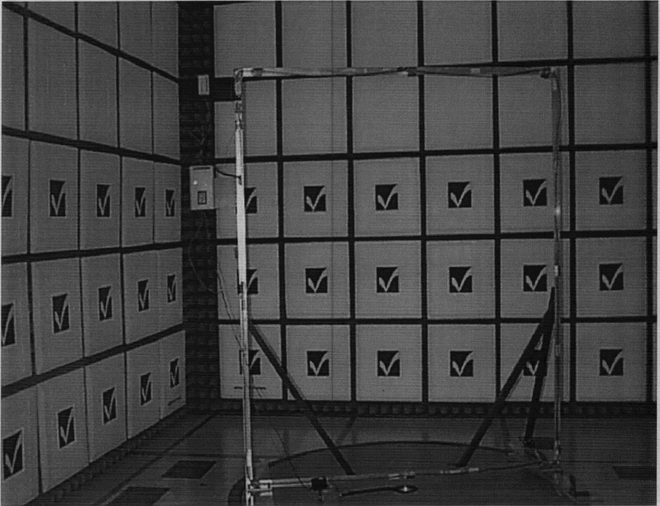
Front view of the LFTX1 mounted on the double loop conductive doorframe during the Radiated Emissions tests.
