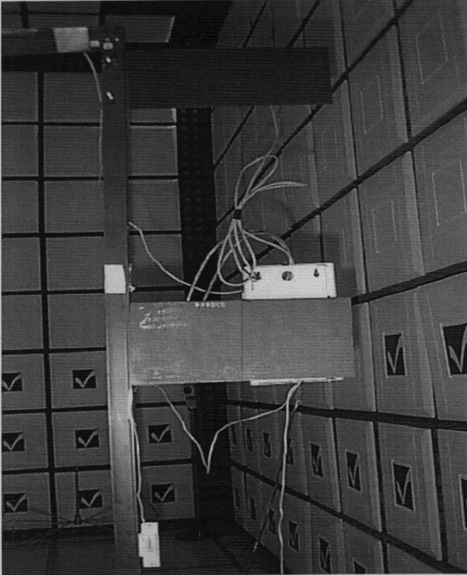
Rear view of the LFTX1 mounted on the single loop non-conductive doorframe during the Radiated Emissions tests.
