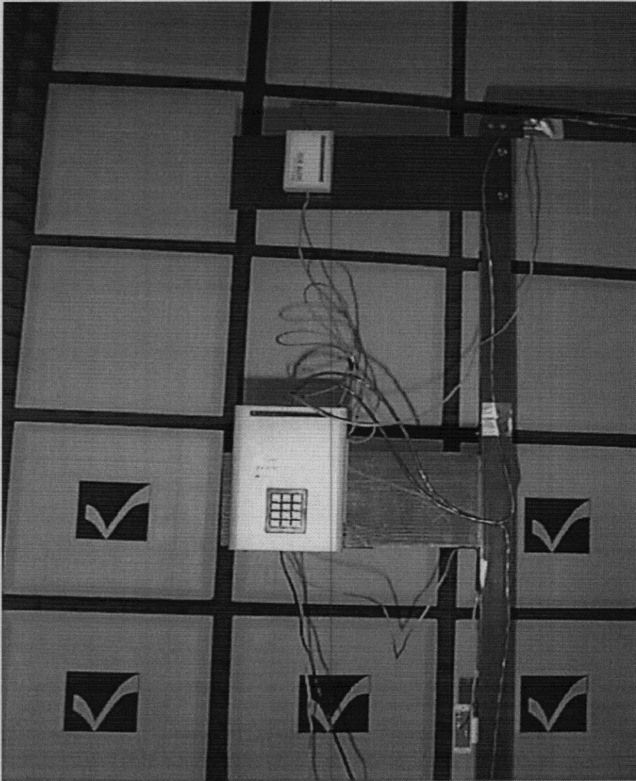
Close up view of the LFTX1 mounted on the single loop non-conductive doorframe during the Radiated Emissions tests.
