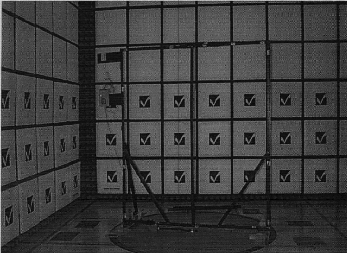
Front view of the LFTX1 mounted on the double loop non-conductive doorframe during the Radiated Emissions tests.
