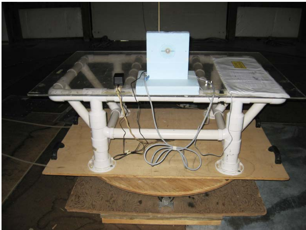
Radiated Back - Below 1GHz
