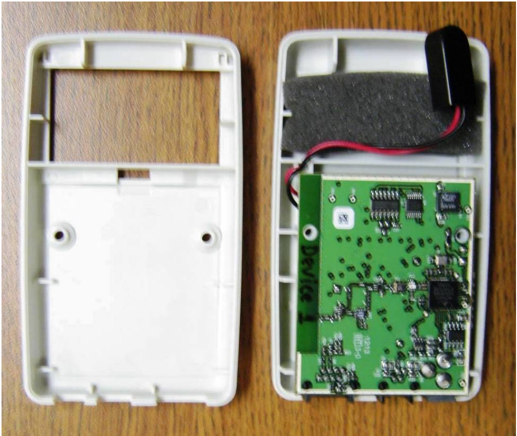
Back Cover Removed
