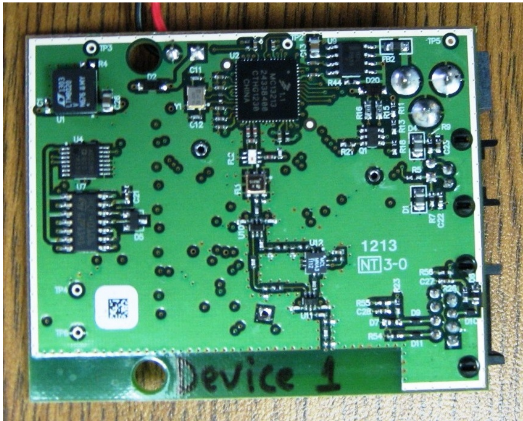
Circuit Board - Side 2
