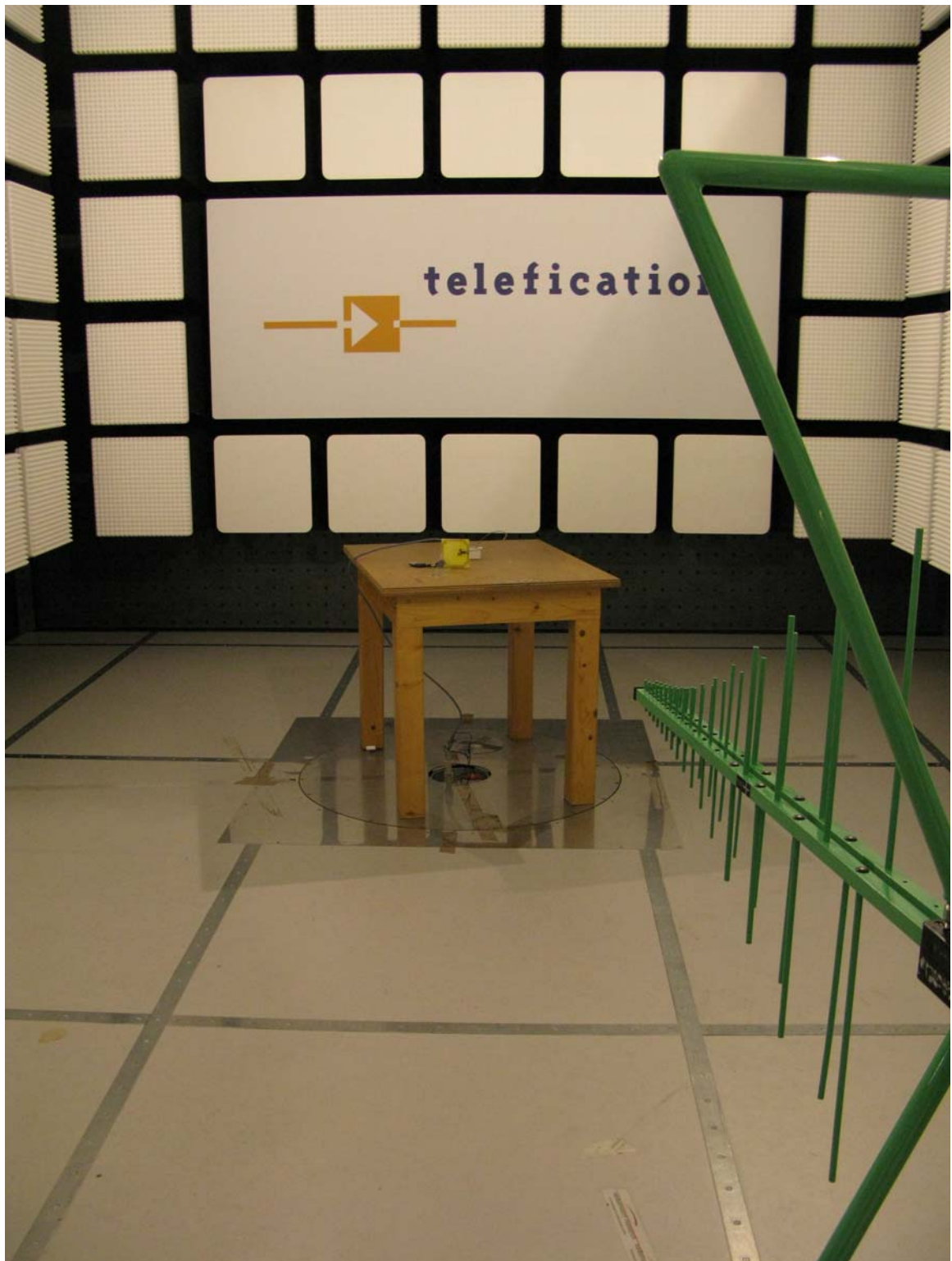
Photograph 2: Test setup radiated emissions ( \geq 30 MHz)
