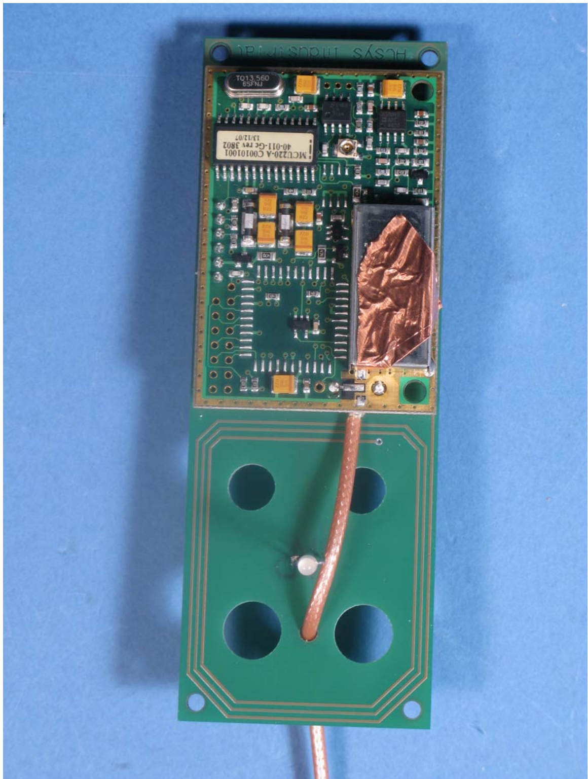
Photograph 1: PCB top view of MR50 reader unit
