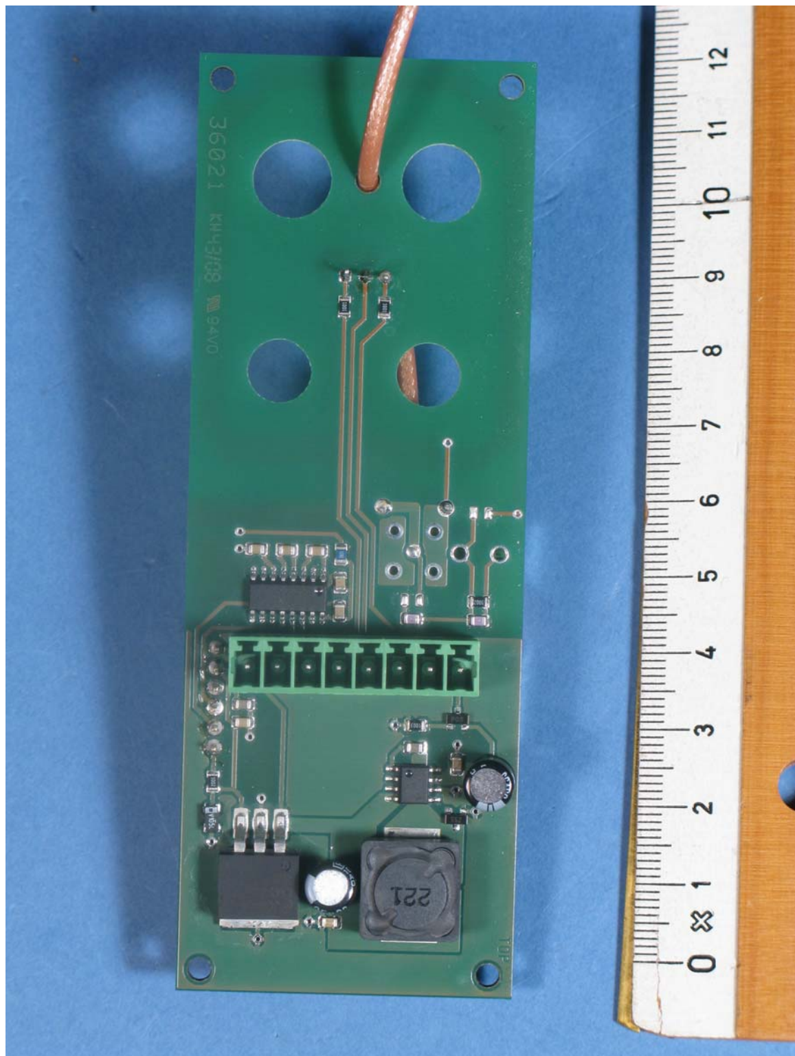
Photograph 2: PCB bottom view of MR50 reader unit
