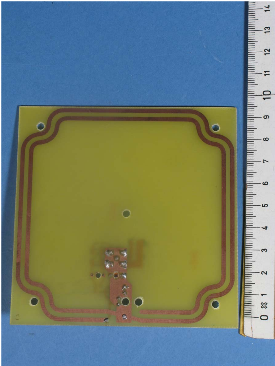
Photograph 4: Bottom view of MR50 PCB antenna
