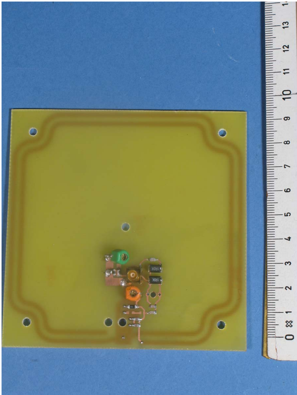
Photograph 3: Top view of MR50 PCB antenna
