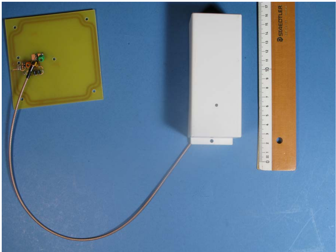
Photograph 1: MR50 System top view
