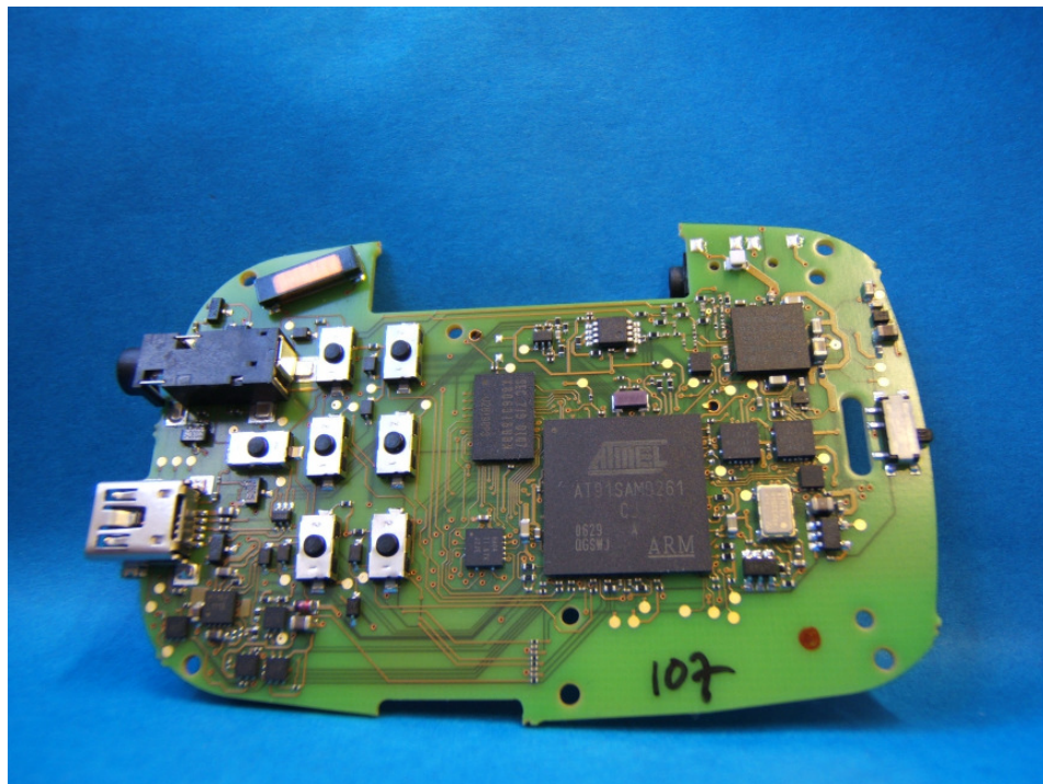
Fig 1 Phonak inspiro PCB top view
