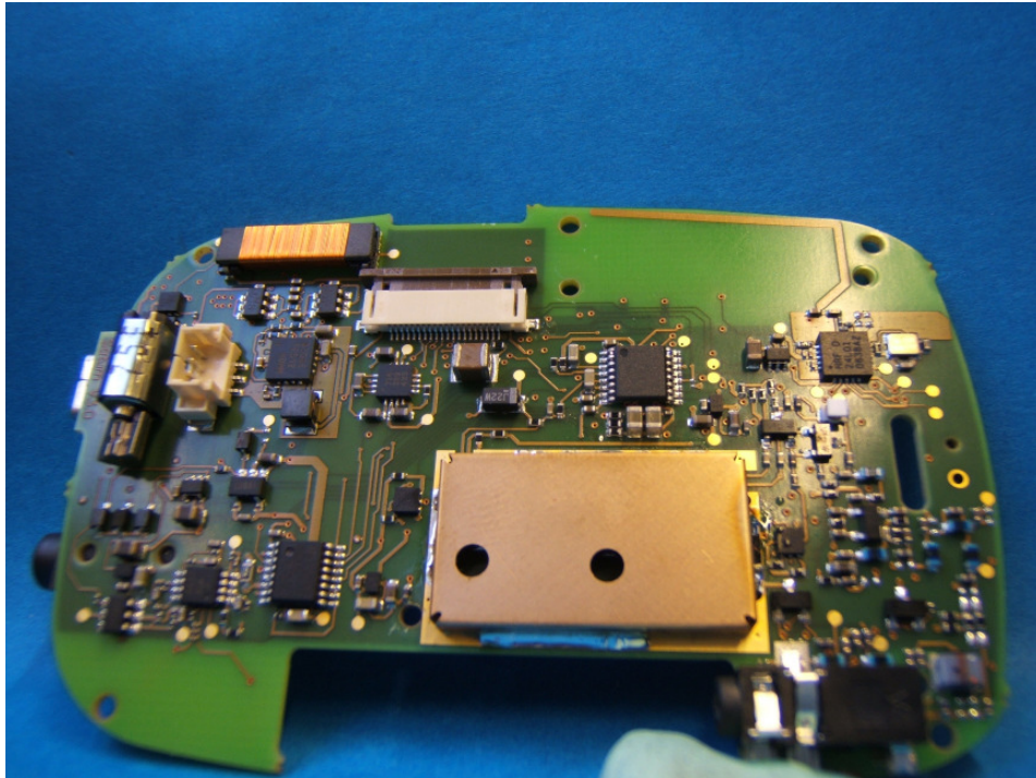
Fig 2 Phonak inspiro PCB bottom view
