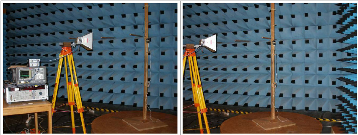
Fig 1 Radiated measurements - carrier
