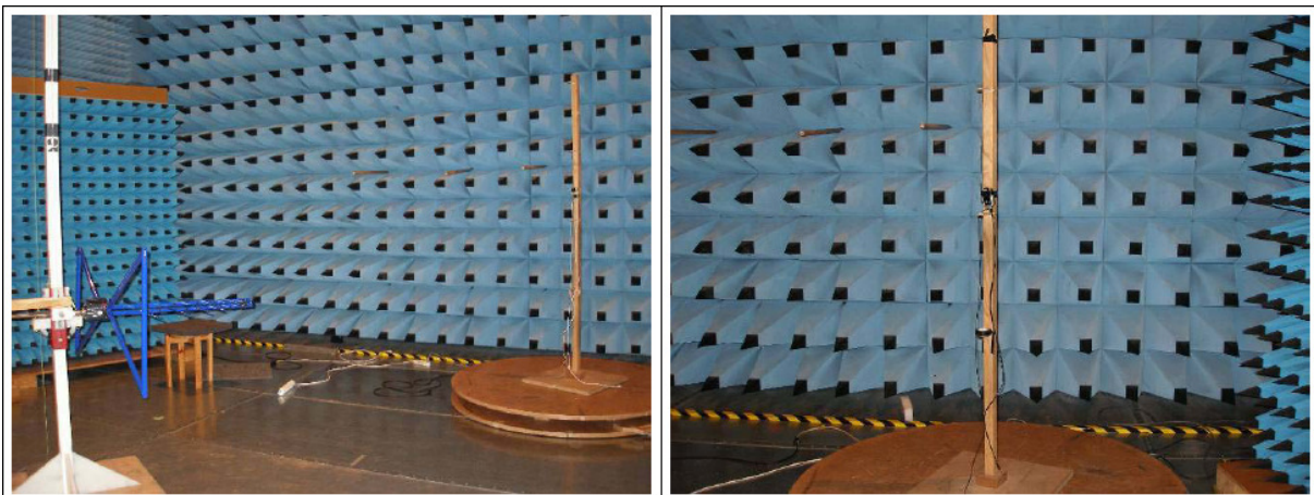
Fig 2 Spurious emissions
