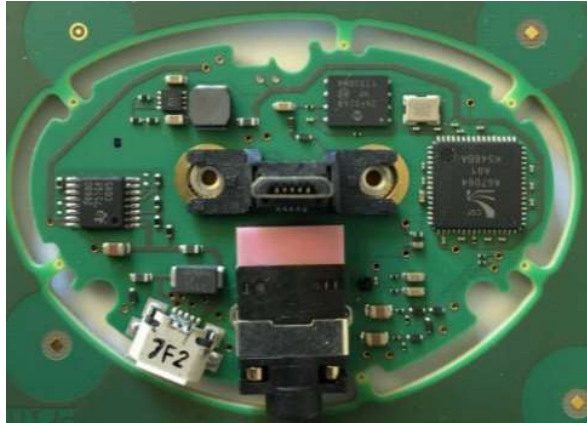
Docking PCB
