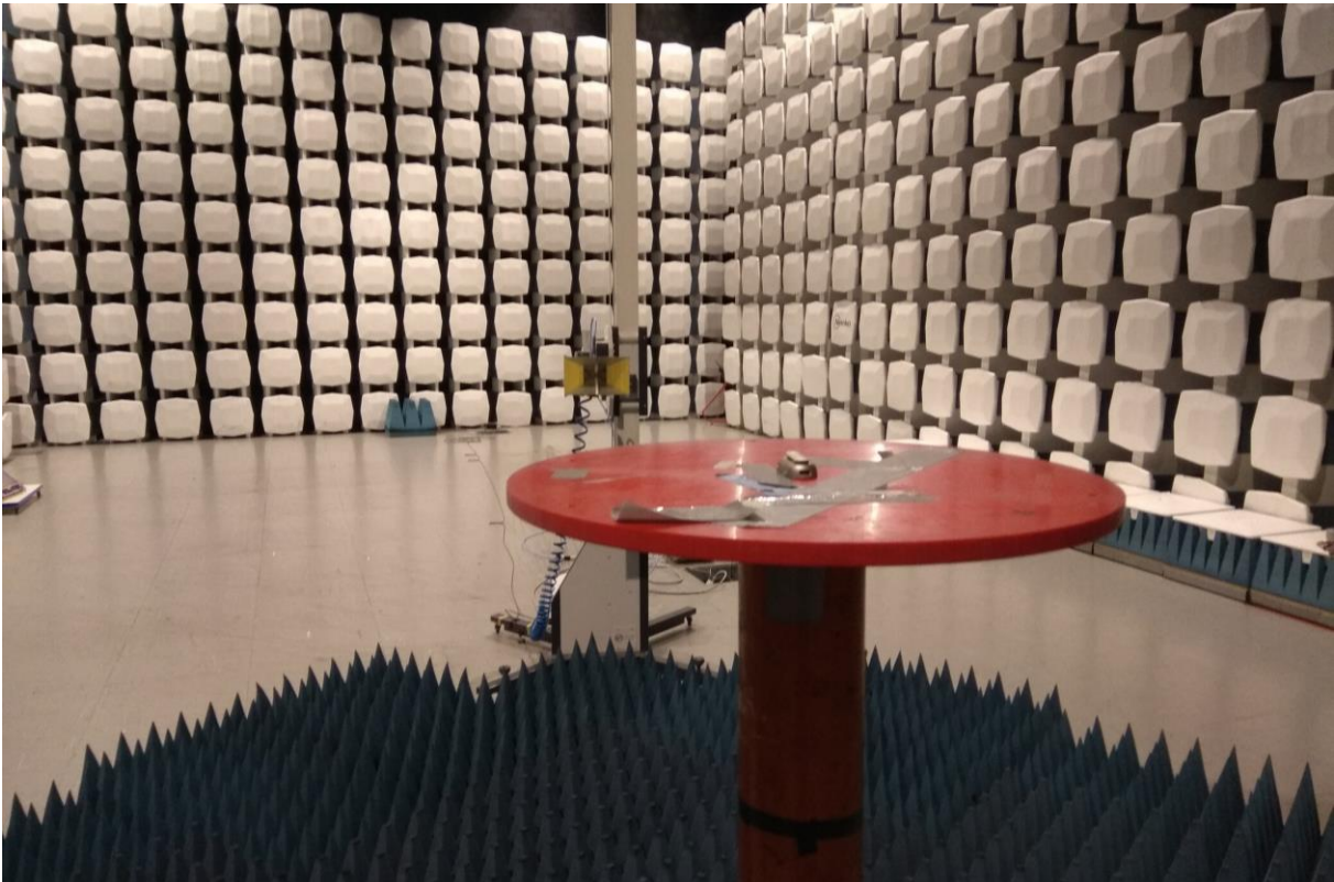
Radiated Emissions, 1 GHz – 18 GHz
