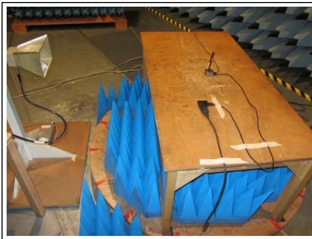
Fig 5 Spurious emissions – 1 GHz- 26.5 GHz
