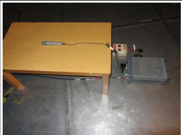
Fig 1 Conducted measurements – interference voltage
