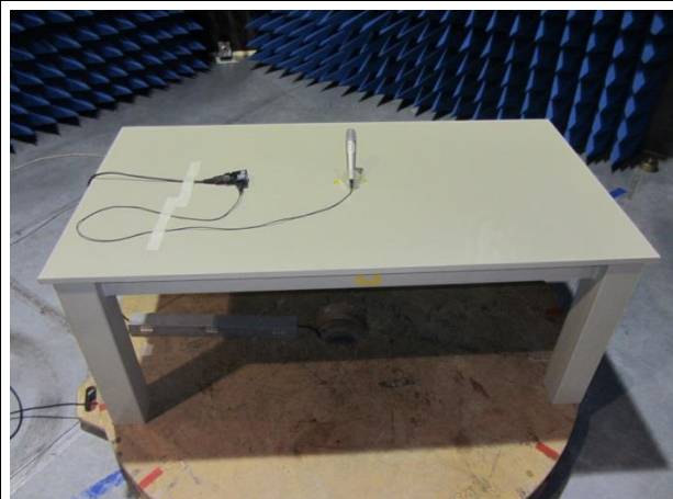
Fig 3 Spurious emissions 9 kHz – 30 MHz
