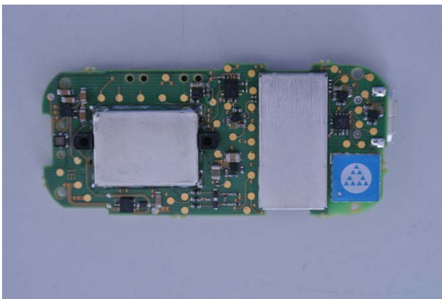
PCB top side without shielding and with shielding
