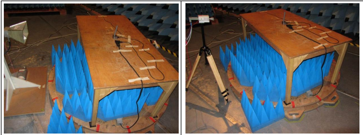
Fig 4 Spurious emissions – 1 GHz- 26.5 GHz
