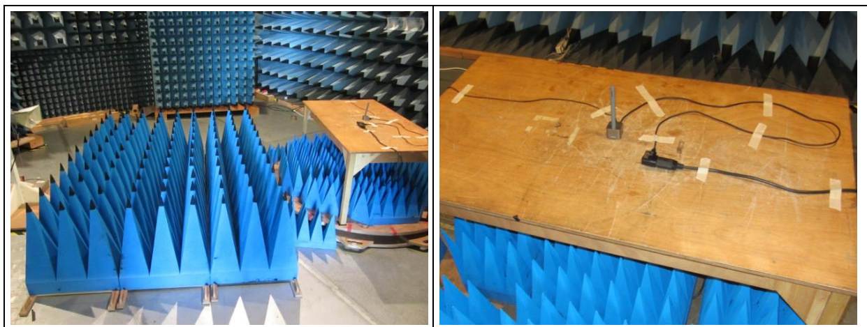
Fig 2 Radiated measurements - carrier
