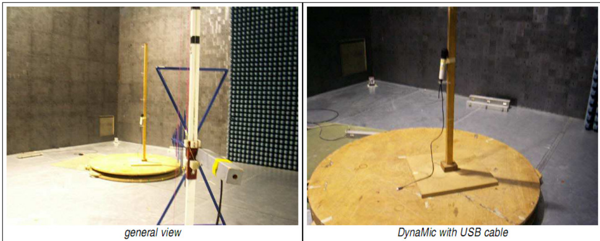
Fig 7 Spurious emissions 30 MHz-1 GHz
