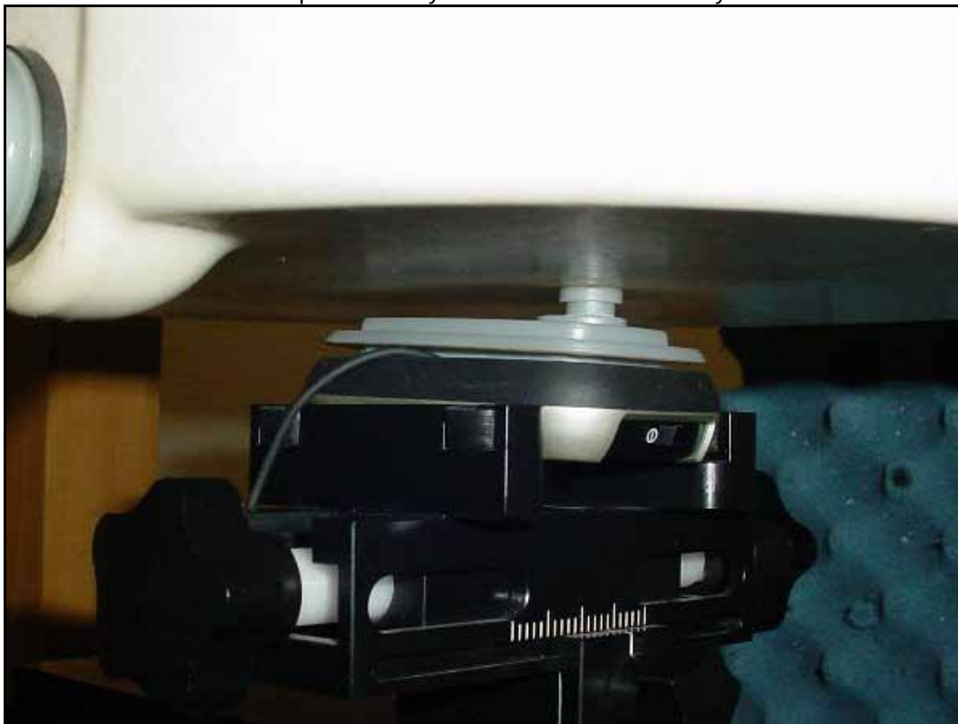
Photo 7: Test position body worn rear side without any distance
