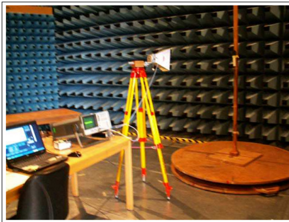
Fig 3 Spurious emissions 1 GHz – 18 GHz
