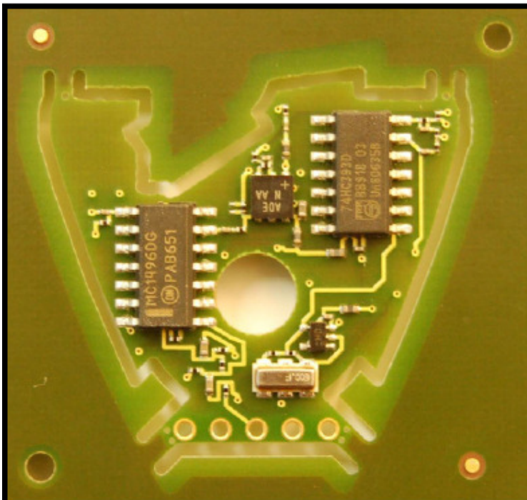
Transmitter electronics – Front Side
