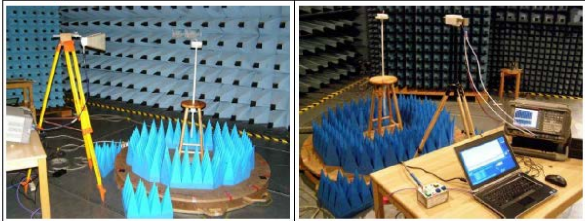
Fig 3 Spurious emissions – 1 GHz- 26.5 GHz
