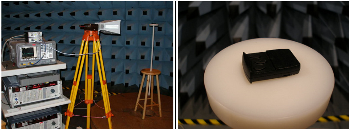
Fig 1 Carrier - radiated measurements
