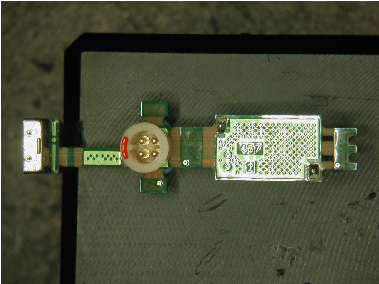
Img 2: Phonak Audéo Yes internal backside view
