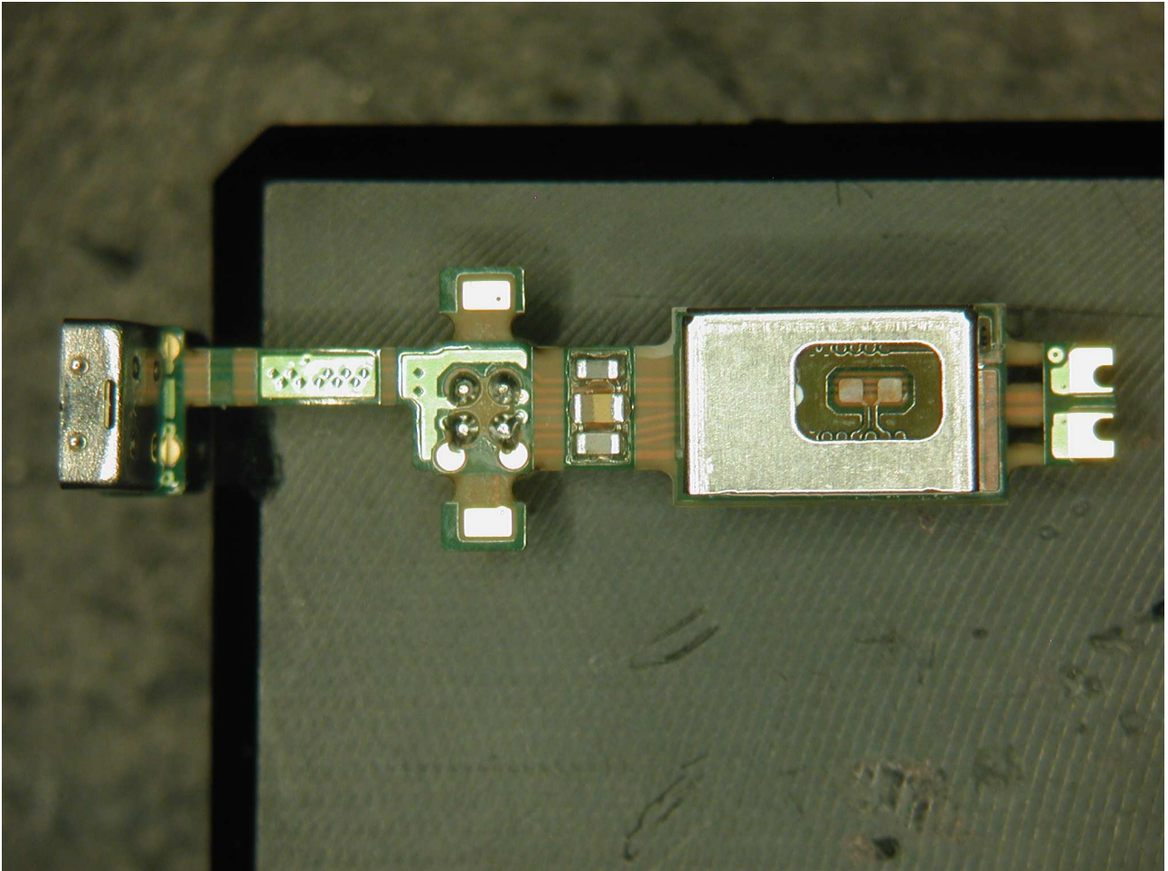
Img 1: Phonak Audéo Yes Internal frontside view
