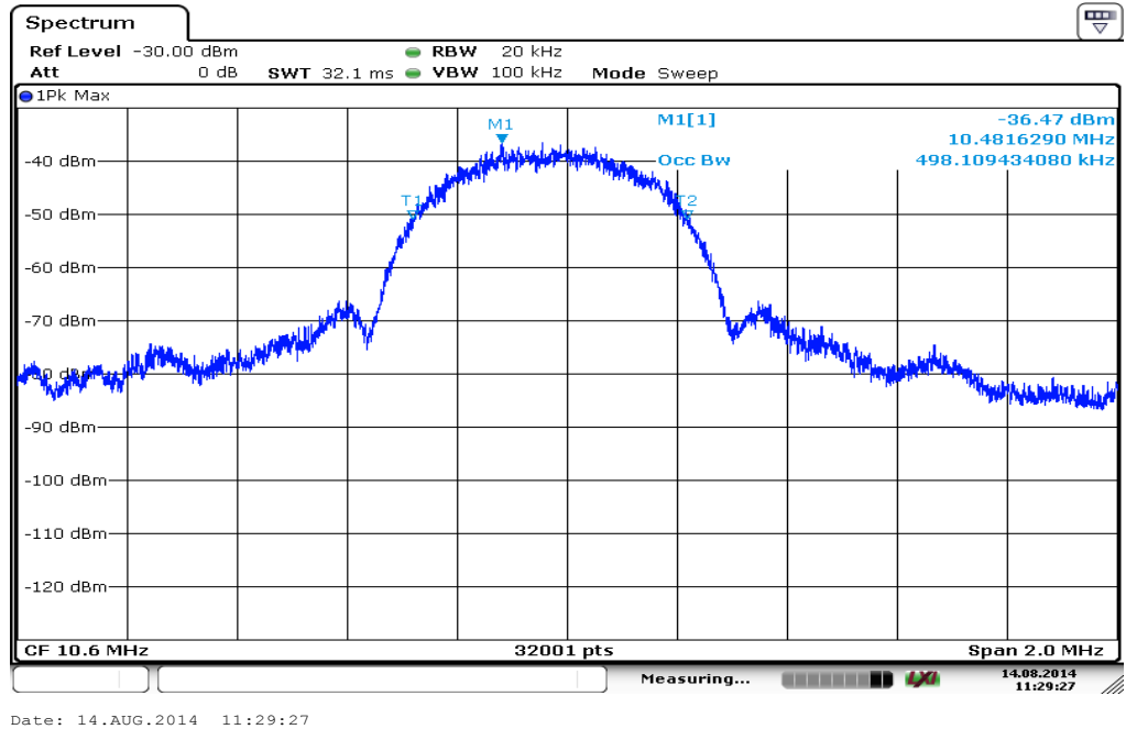
Plot 1: OBW (99 % - bandwidth)
