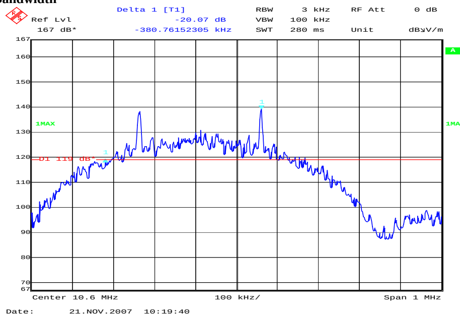
Plot 3 20 dB-Bandwidth
