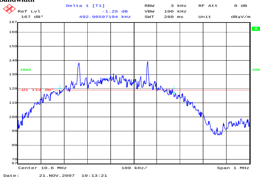
Plot 2: 20 dB-Bandwidth
