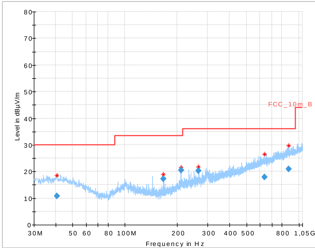
Plot 2: 30 MHz – 1 GHz, vertical and horizontal polarisation, Palio 2
