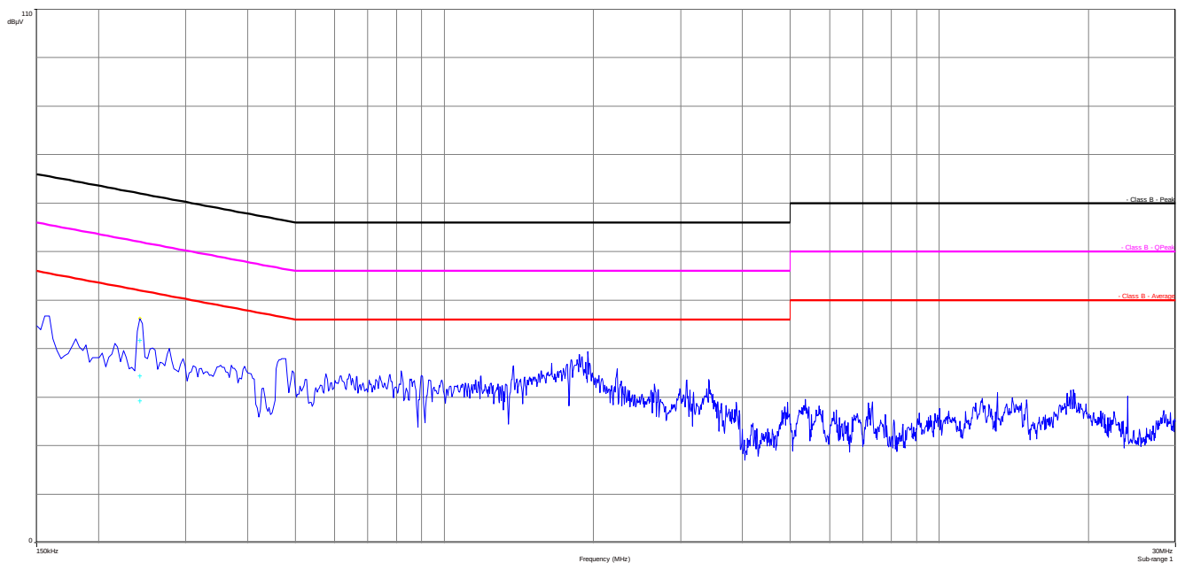
Plot 4: 150 kHz to 30 MHz, neutral line, Palio 3
