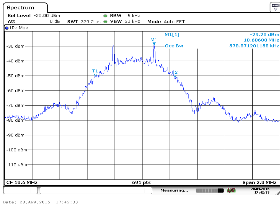
Plot 1: 99 % emission bandwidth, Palio 2
