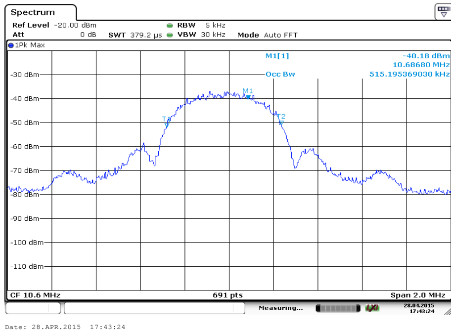
Plot 2: 99 % emission bandwidth, Palio 3
