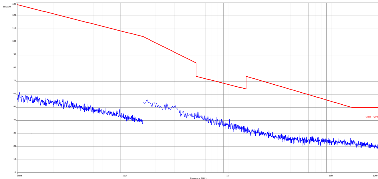
Plot 3: 9 kHz – 30 MHz, magnetic emissions, Palio 3
