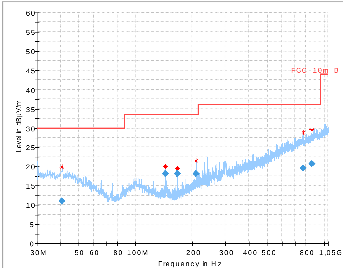
Plot 4: 30 MHz – 1 GHz, vertical and horizontal polarisation, Palio 3
