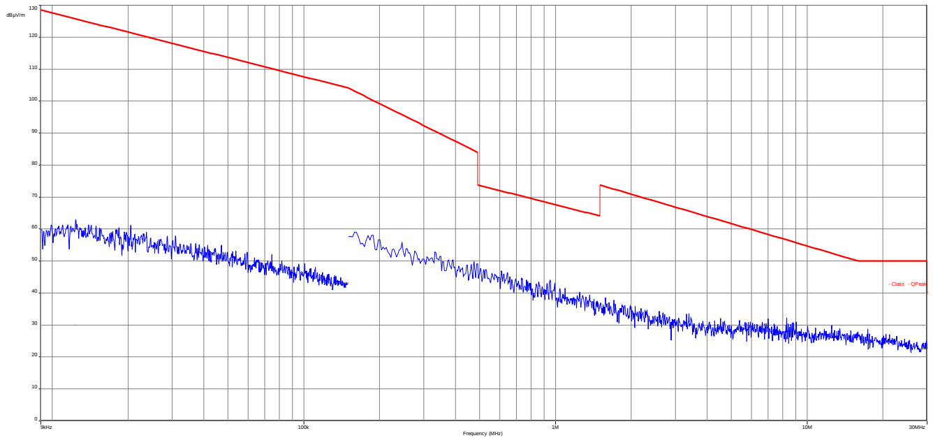
Plot 1: 9 kHz – 30 MHz, magnetic emissions, Palio 2
