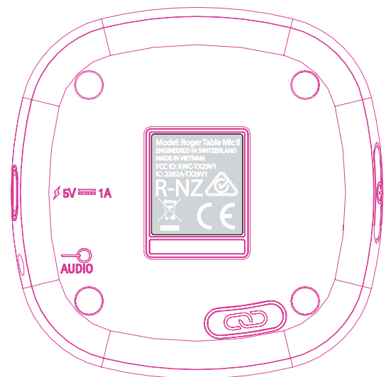
Placement of label. Scale 1:1
