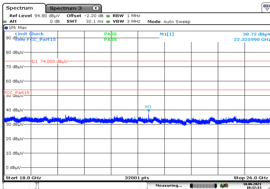
Plot 6: 18 GHz to 26 GHz, TX mode, high channel, vertical & horizontal polarization
