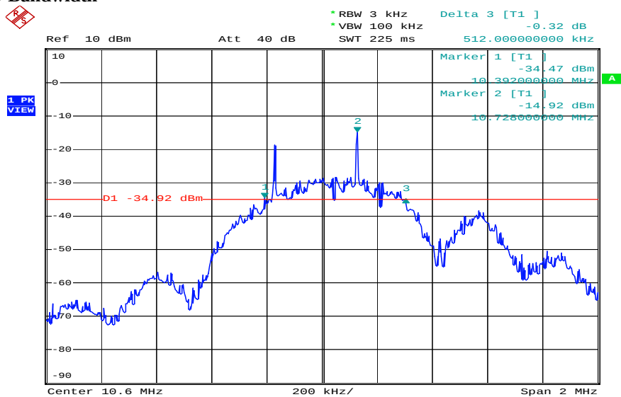
Plot 1: 20 dB-Bandwidth
