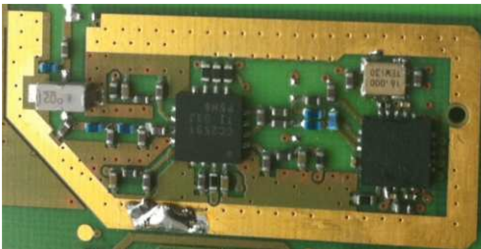
2.4GHz components
