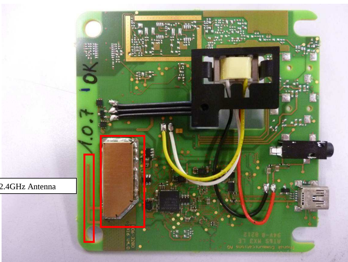
2.4GHz Transmitter
