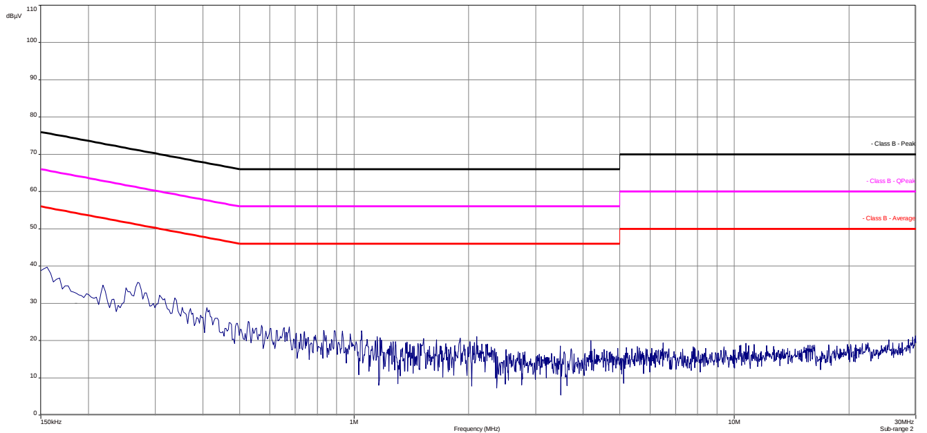
Plot 3: 150 kHz to 30 MHz, TX mode, phase line with external antenna
