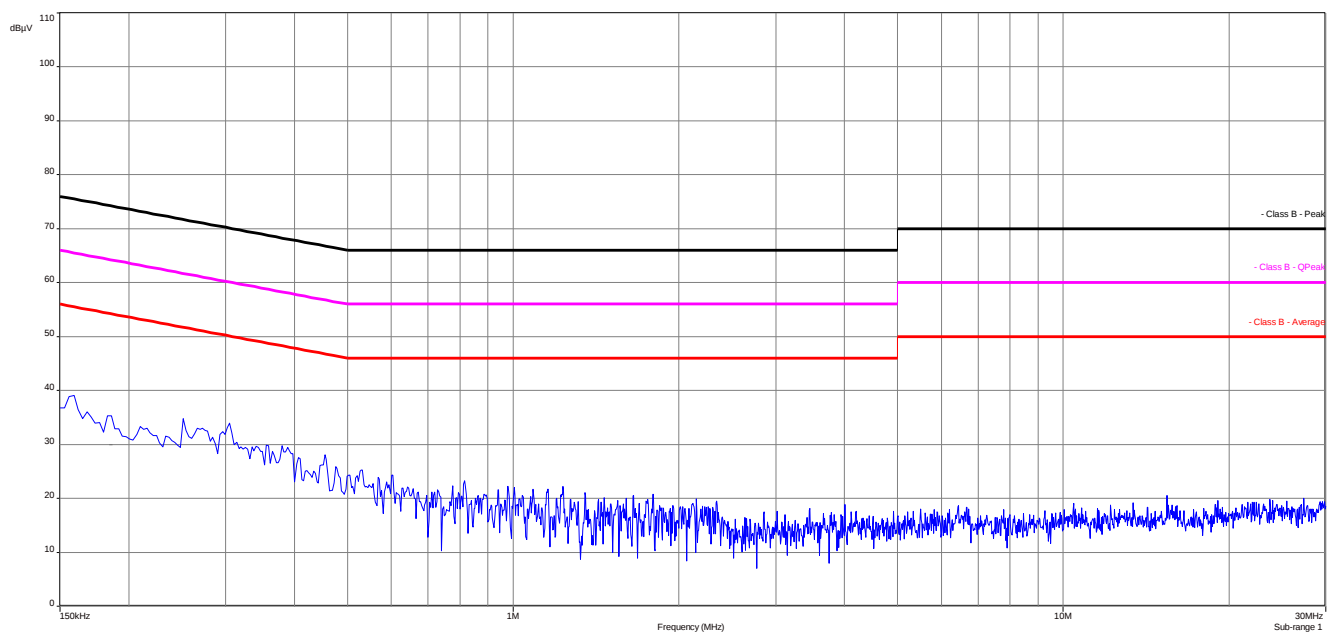
Plot 4: 150 kHz to 30 MHz, TX mode, neutral line with external antenna
