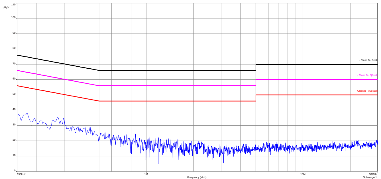
Plot 2: 150 kHz to 30 MHz, TX mode, neutral line with internal antenna
