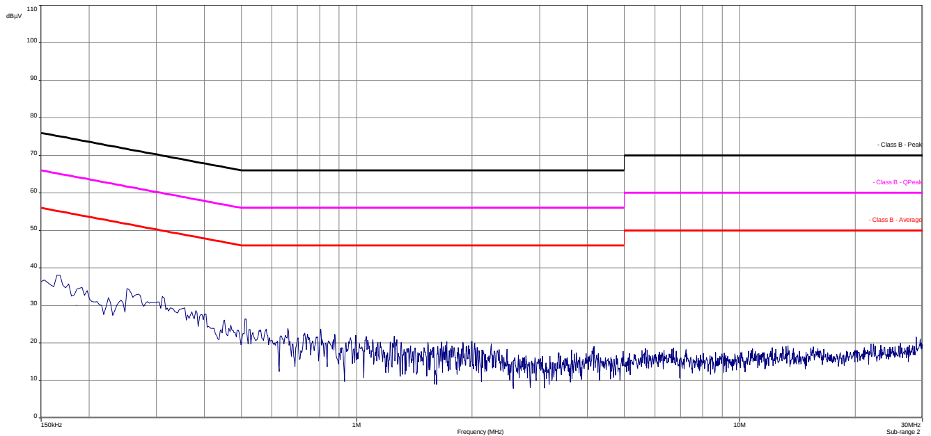
Plot 1: 150 kHz to 30 MHz, TX mode, phase line with internal antenna
