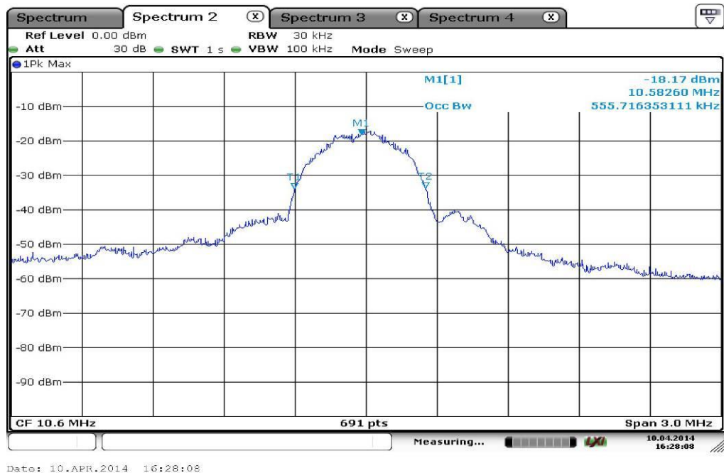
Plot 1: 99% bandwidth, integrated ferrite antenna
