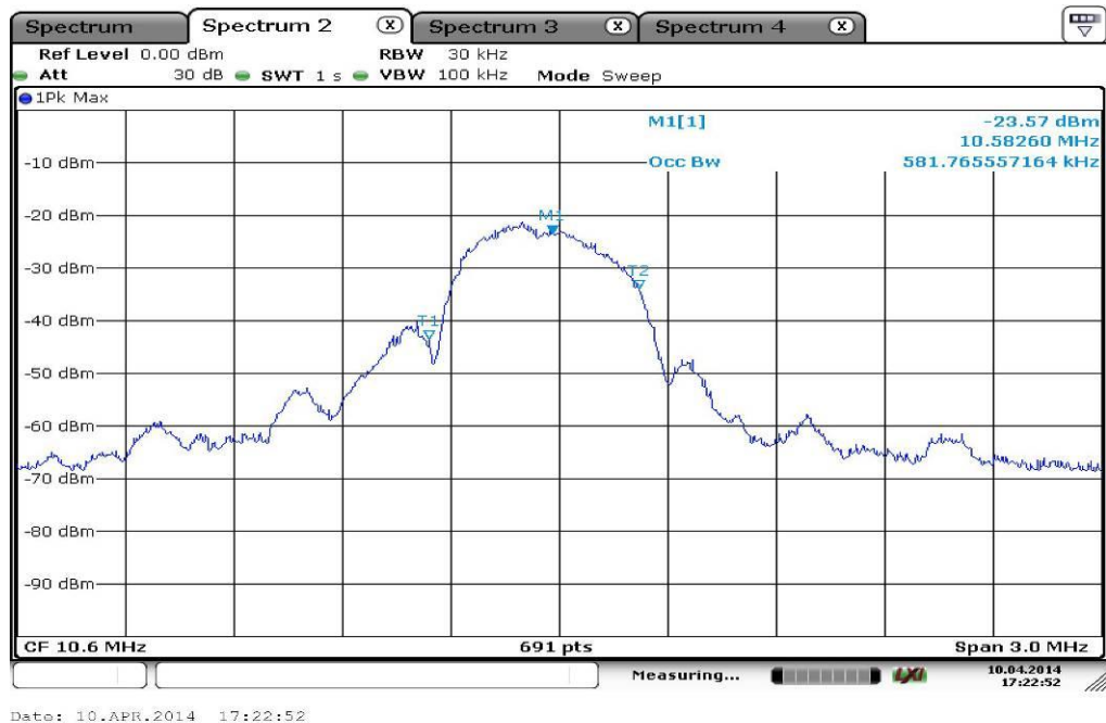
Plot 2: 99% bandwidth, neck loop antenna
