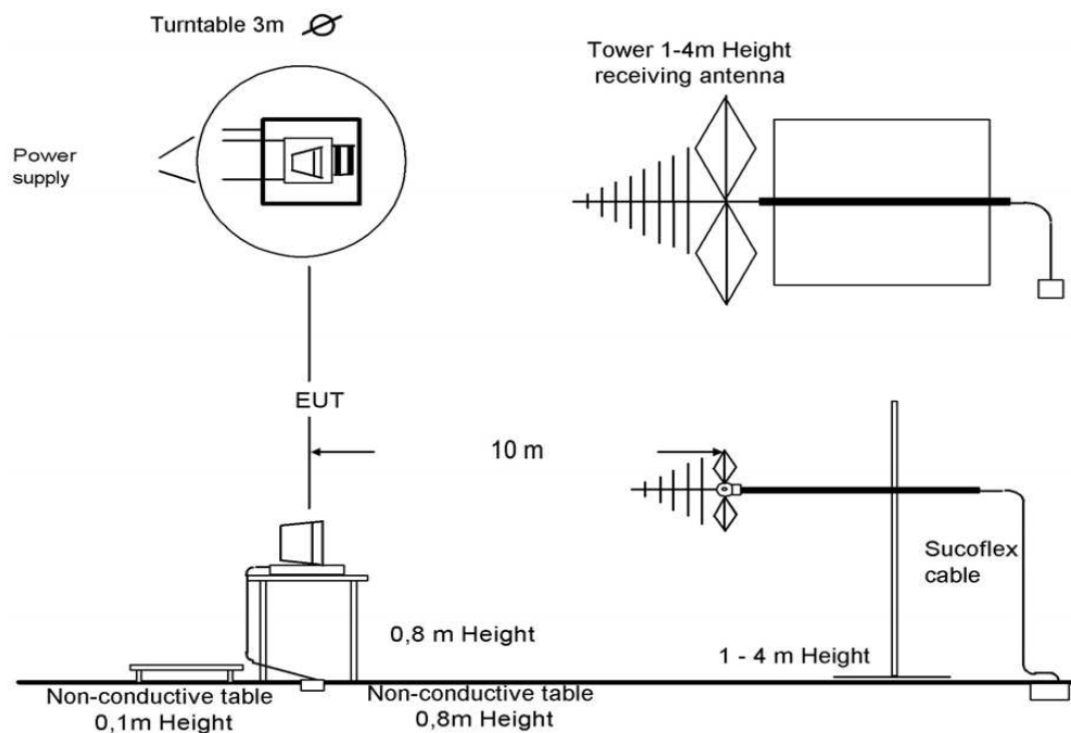
Picture 1: Diagram radiated measurements
