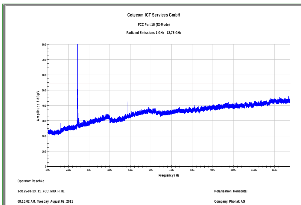
Plot 7: 1 GHz to 12.75 GHz, TX mode, channel 39, horizontal polarization
