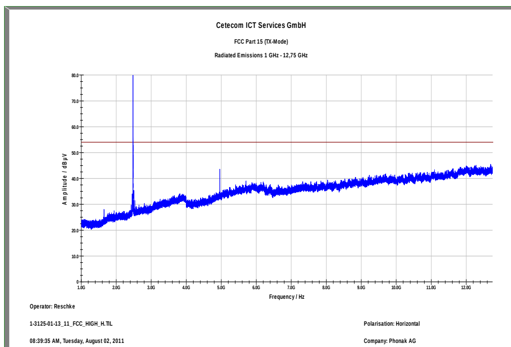
Plot 11: 1 GHz to 12.75 GHz, TX mode, channel 78, horizontal polarization
