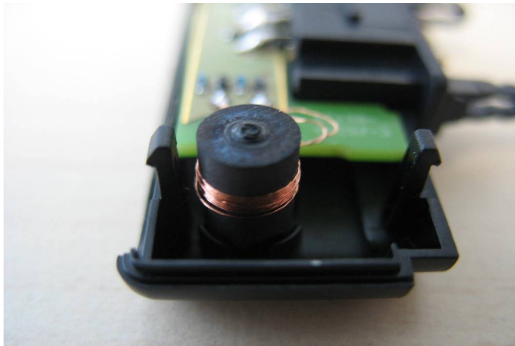
Photo 6: antenna
