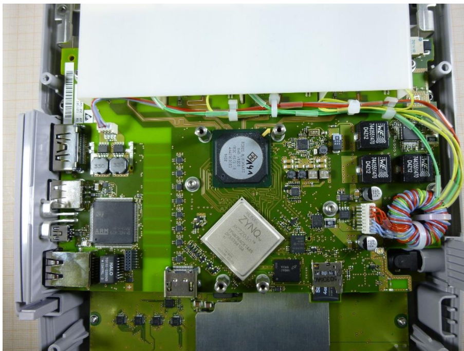
Photo 6: PCB
