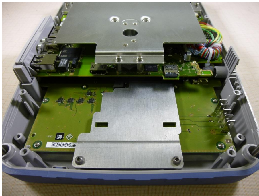
Photo 3: Bottom view
