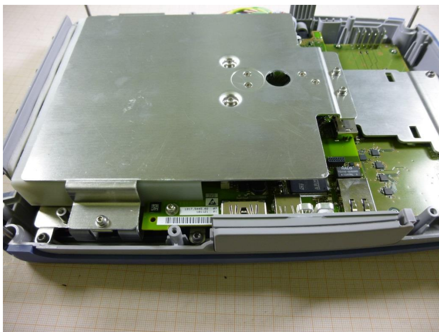
Photo 4: Connector side
