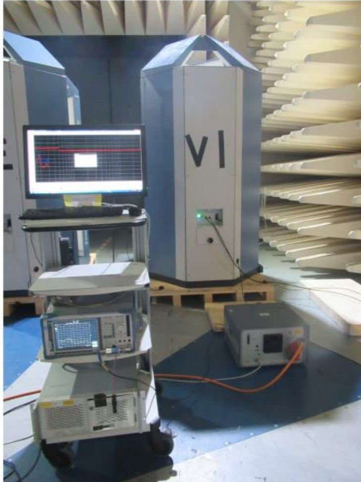
Test Setup Photos FCC 15B Extract from Test Report 80119127-03 issued by CSA Group Bayern GmbH
