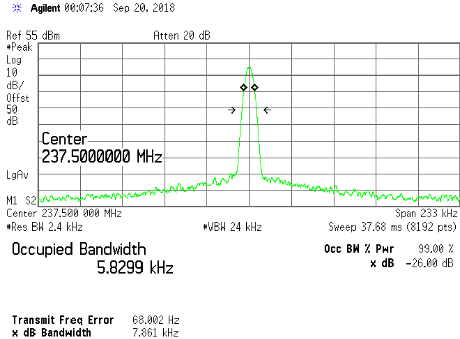
Figure 2: Occupied Bandwidth Low Channel
