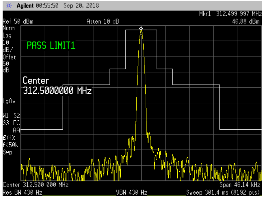
Figure 11. Conducted Spurious Emissions, High Channel Mask
