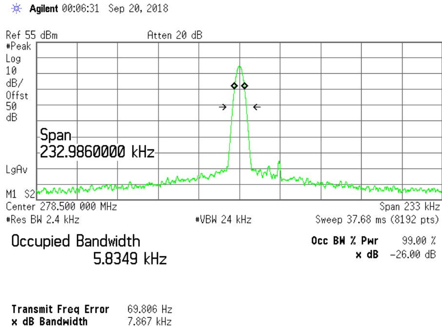
Figure 3. Occupied Bandwidth Center Channel
