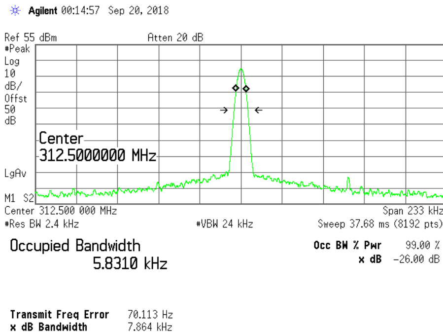
Figure 4: Occupied Bandwidth High Channel
