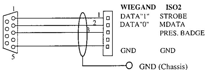
Wiring diagram
