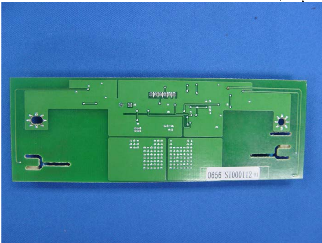
Figure 15 Power Board, Component Side
