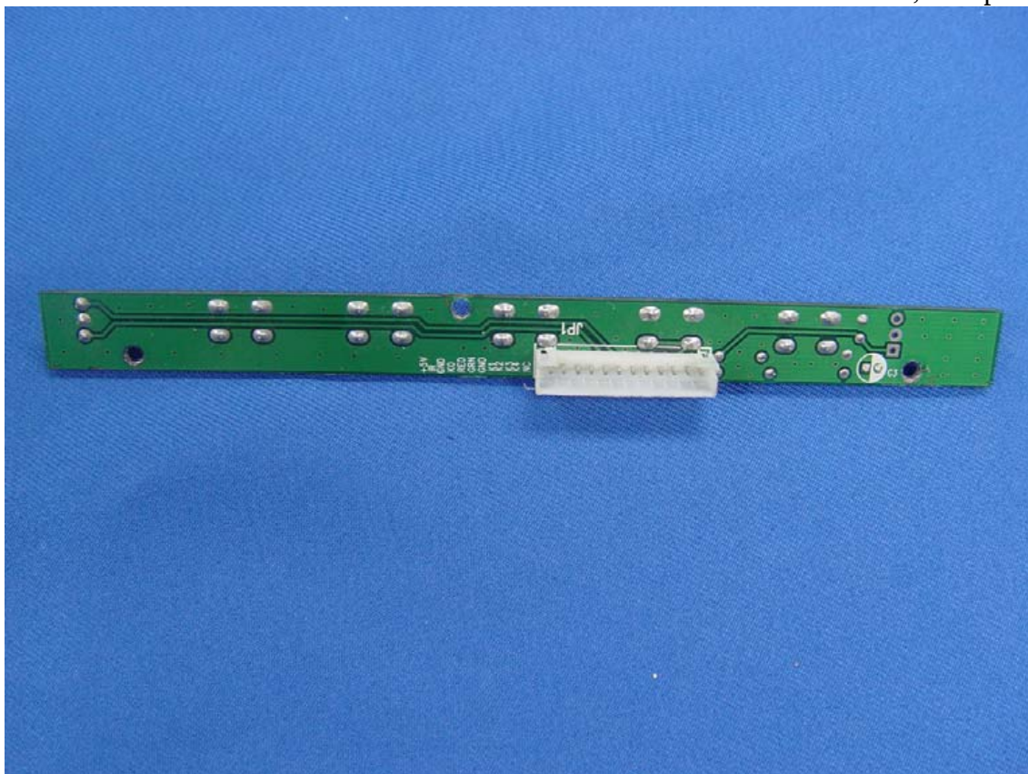
Control Board, Component Side
