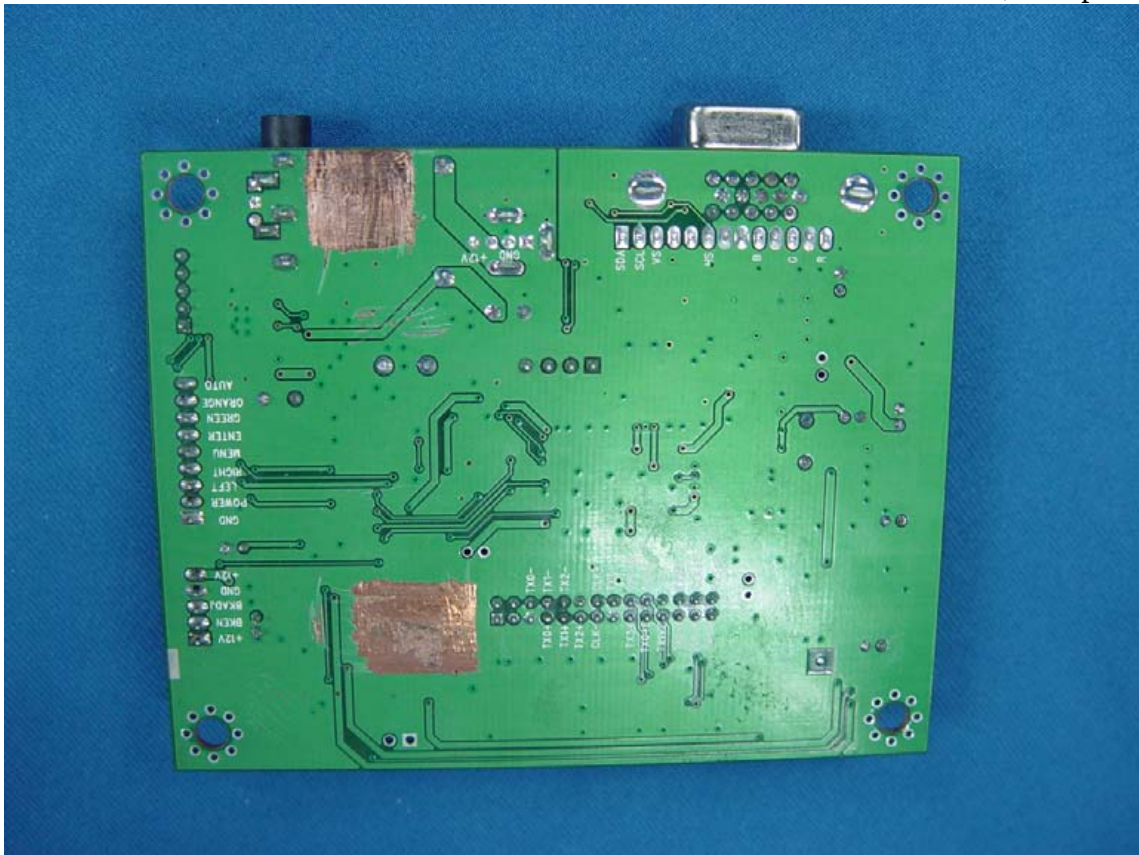
Figure 13 Main Board, Component Side
