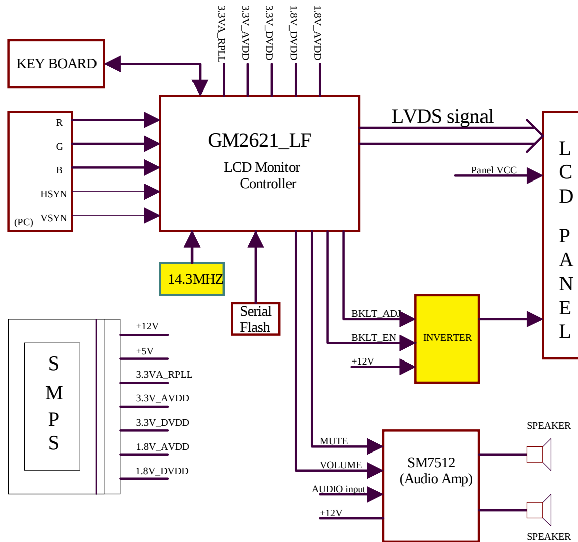
KSAI LCD Monitor Block Diagram
