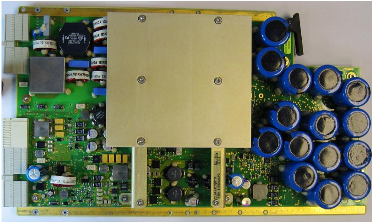
Figure 1: SDU Power Supply Module (PSM) Top
