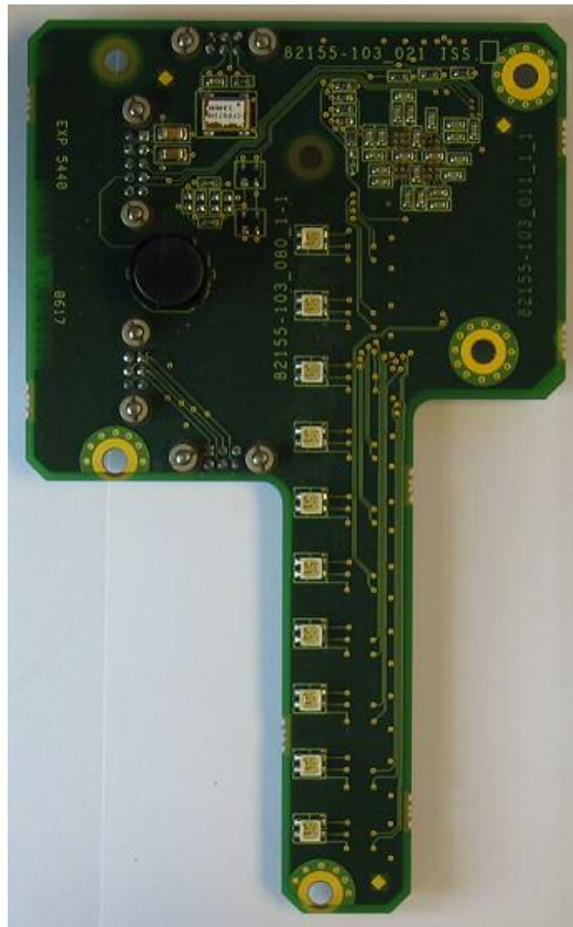
Figure 4: SDU Front Panel Board Top
