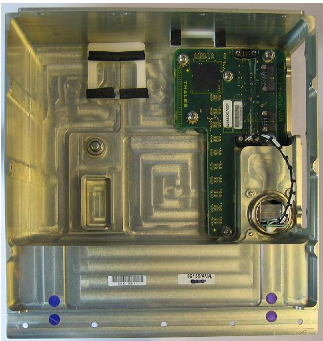
Figure 3: SDU Front Panel Board Assembly
