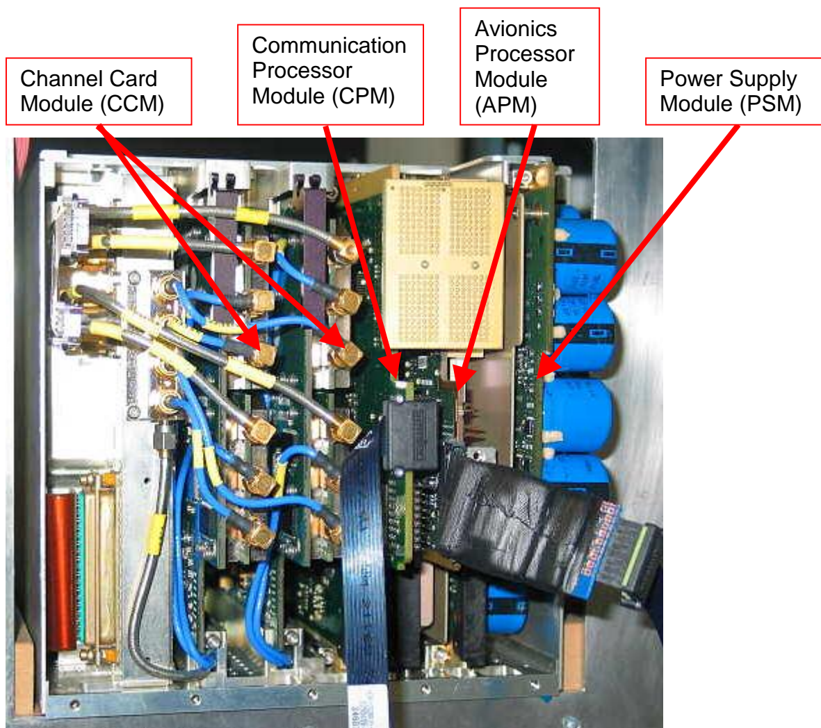
Figure 6: SDU Chassis With PCBs In Place
