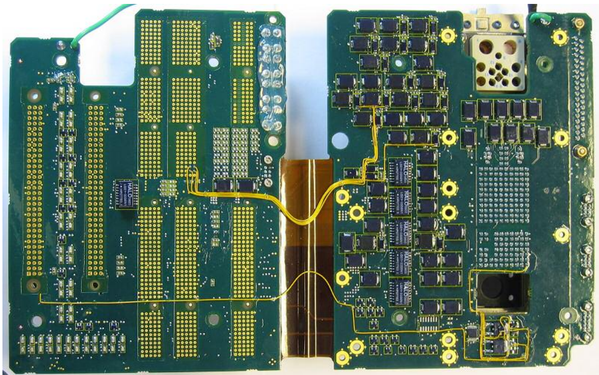
Figure 4: SDU Backplane Bottom
