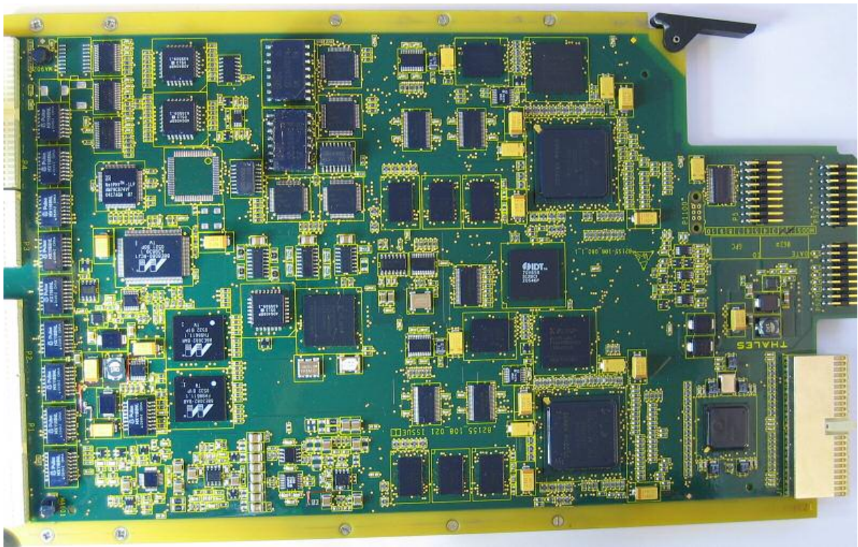
Figure 1: SDU Communication Processor Module (CPM) Top
