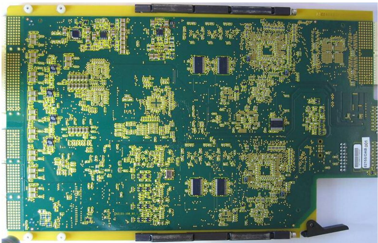
Figure 2: SDU Communication Processor Module (CPM) Bottom
