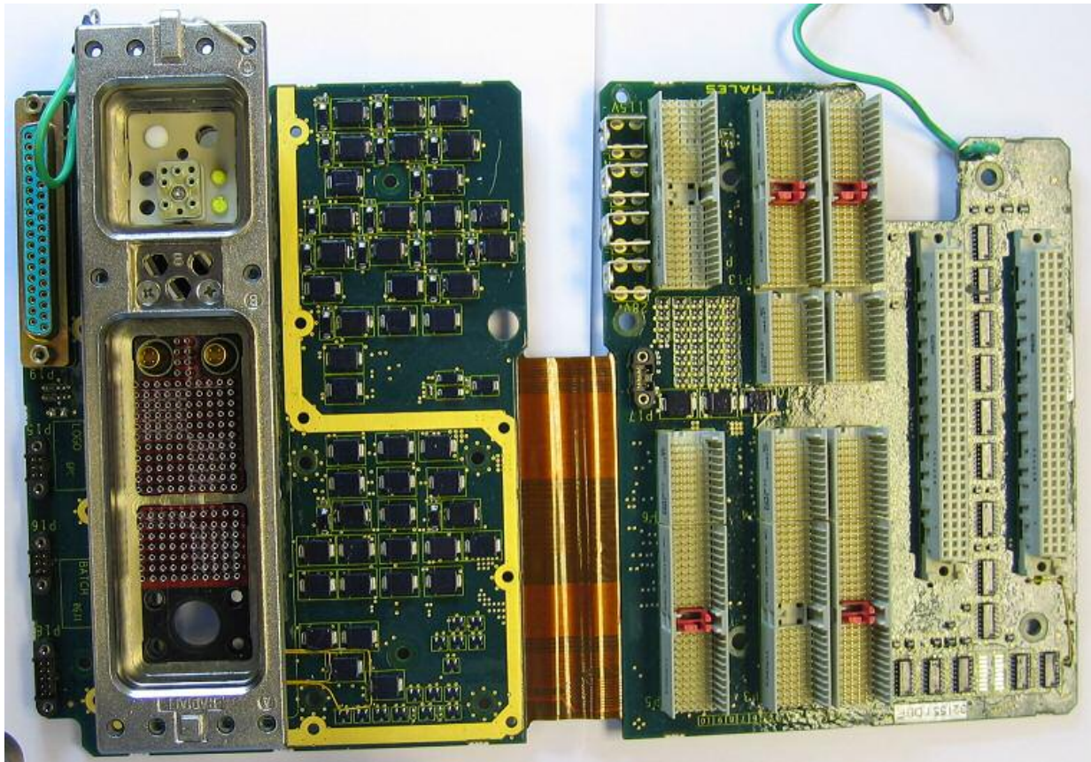
Figure 3: SDU Backplane Top
