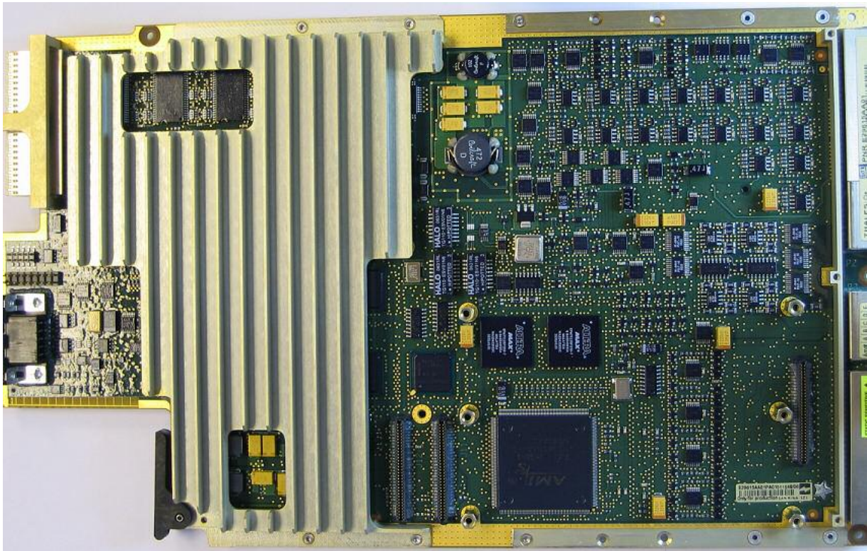
Figure 1: SDU Avionics Processor Module (APM) Top
