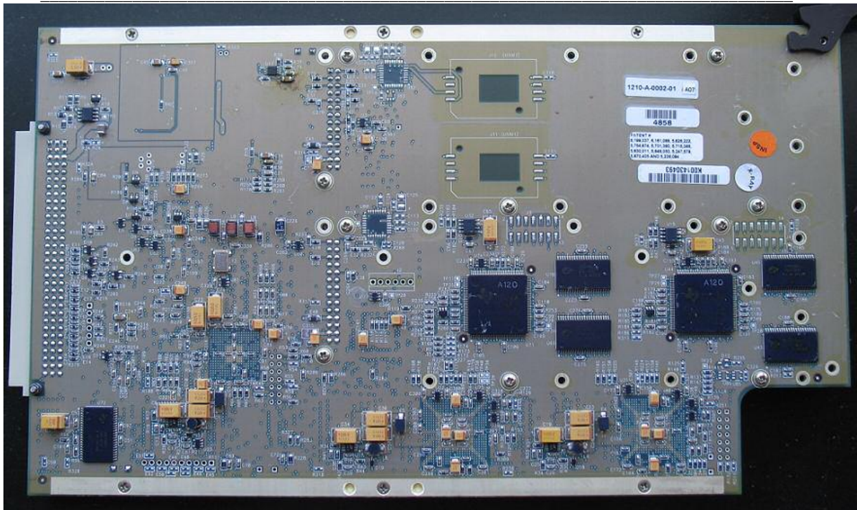
Figure 5: SDU Channel Card Module (CCM) Bottom
