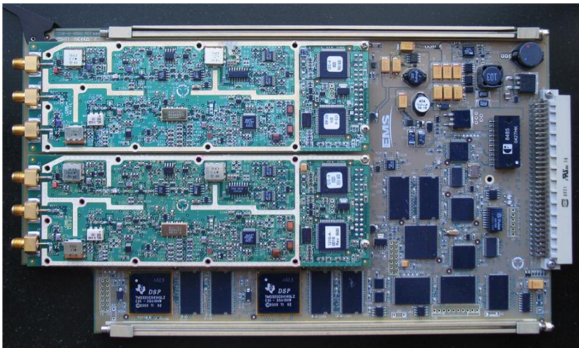
Figure 3: SDU Avionics Processor Module (APM) Bottom
