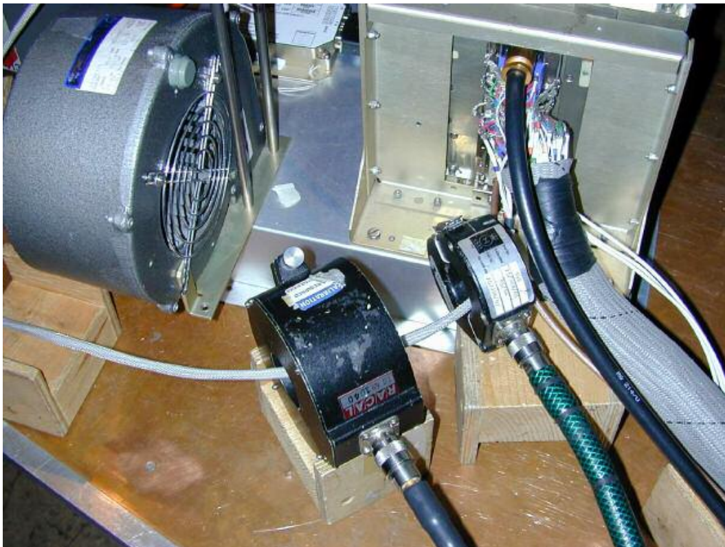
Figure 2: Conducted Susceptibility
